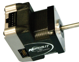
MDO•17 MDrive Plus Speed Control products: integrated NEMA17 motor and controls, IP20-rated
